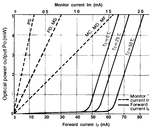
Fig. 52-2 Optical Power Output vs. Forward Current and Monitor Current
