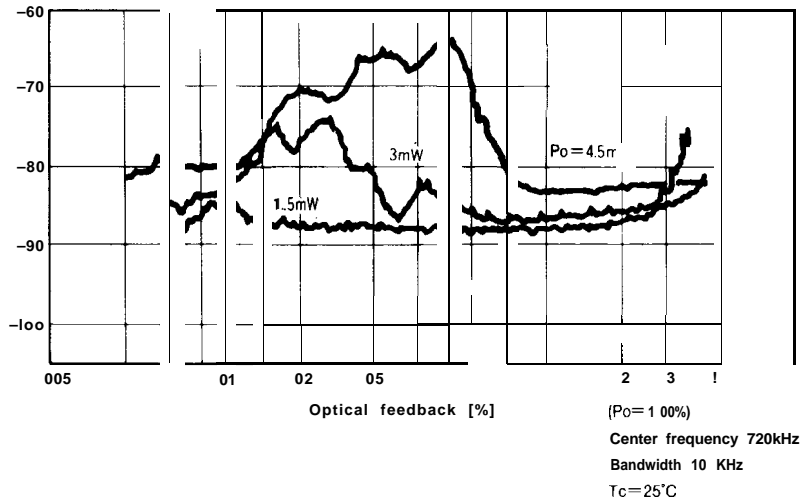
Fig. 53-1 SIN vs. Optical Feedback
