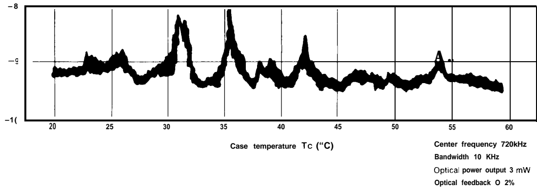
Fig. 53-2 S/N vs. Temperature
